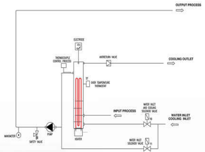
Open Tank Water Unit Diagram WDC
