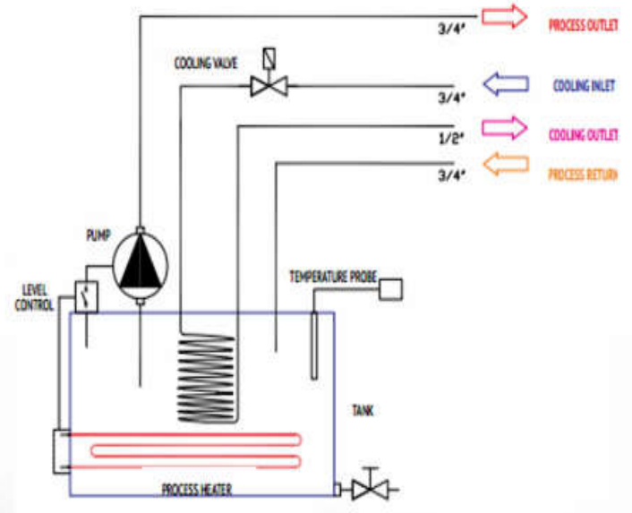
Open Tank Oil Unit Diagram
