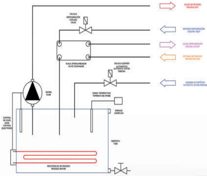
Open Tank Water Unit Diagram
