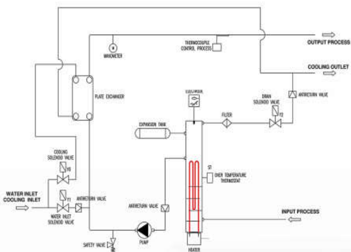
Open Tank Water Unit Diagram WIC
